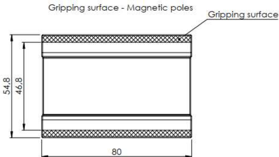
Figure 1. The gripping surface and magnetic poles of MRP-31FK.
