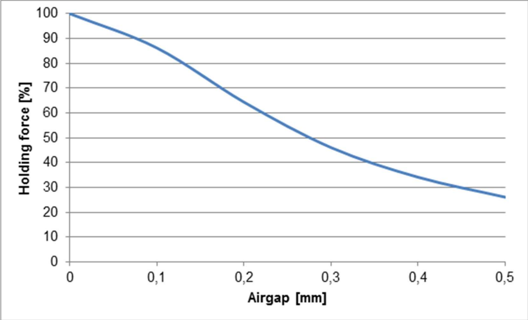
Figure 3. MRP-31FK holding force in proportion to airgap
