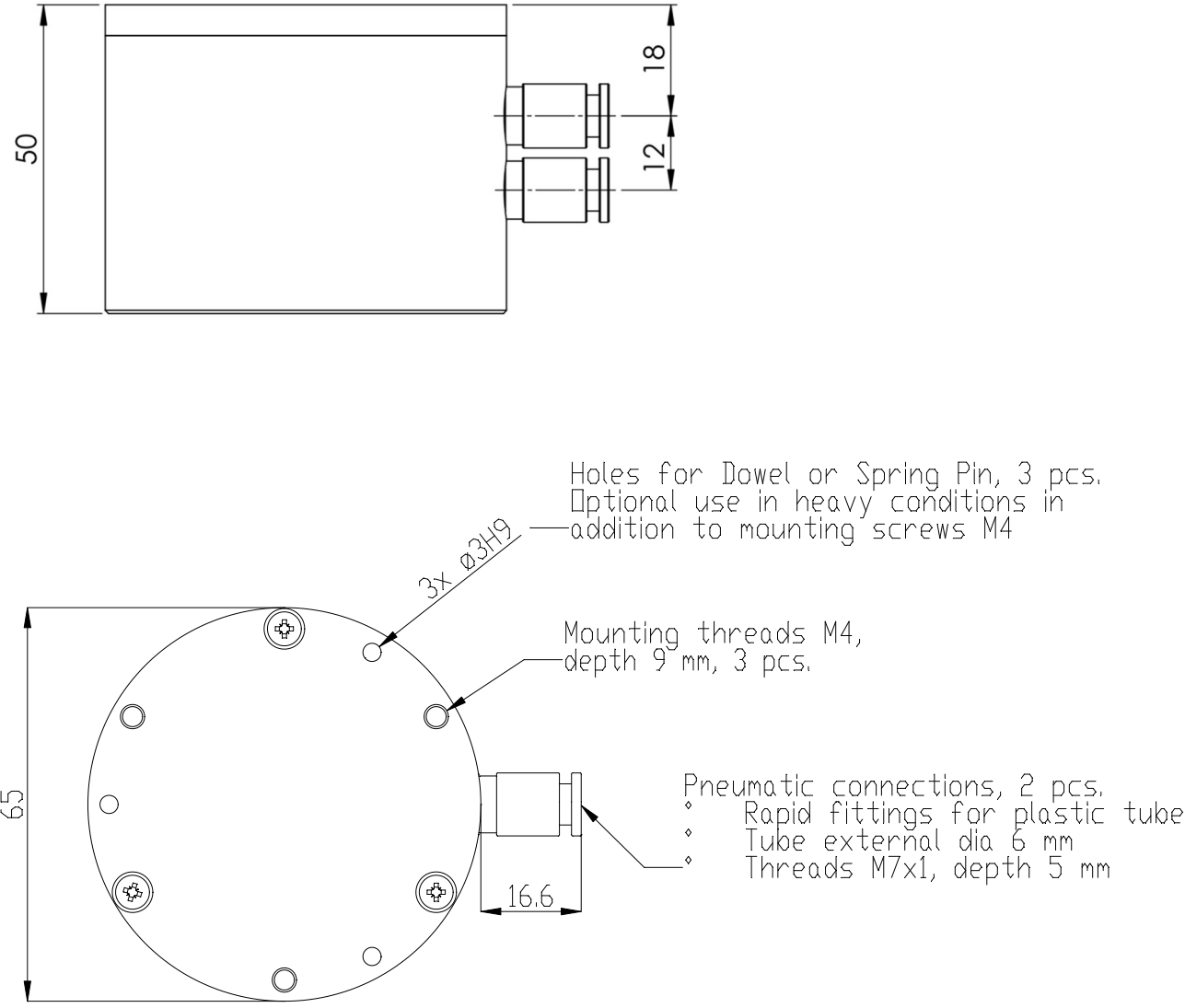
Figure 4. Mounting dimensions of MAP-40.
